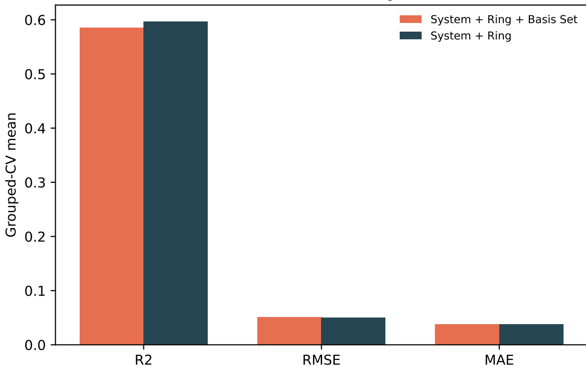
Ablation: norm, |Q_2|_{\text{ring}} atoms
